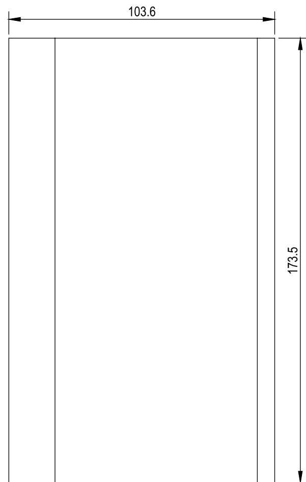
BOARD (K) VERTICAL BRACE
