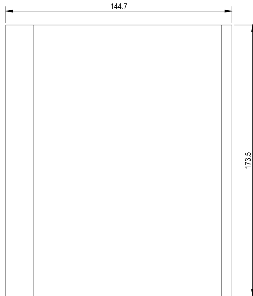
BOARD (L) VERTICAL BRACE
