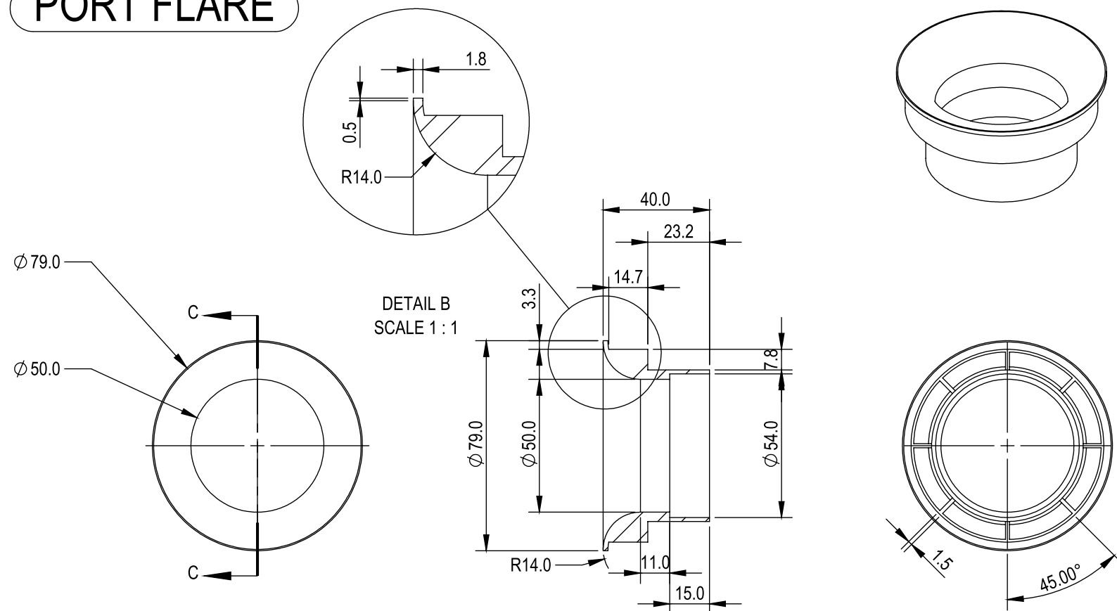
SECTION C-C
